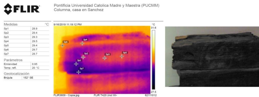
Fig.4. Thermography of a piece of columns.
